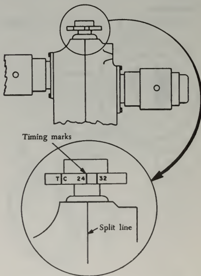
FIGURE 4-28. Propeller flange timing marks.
